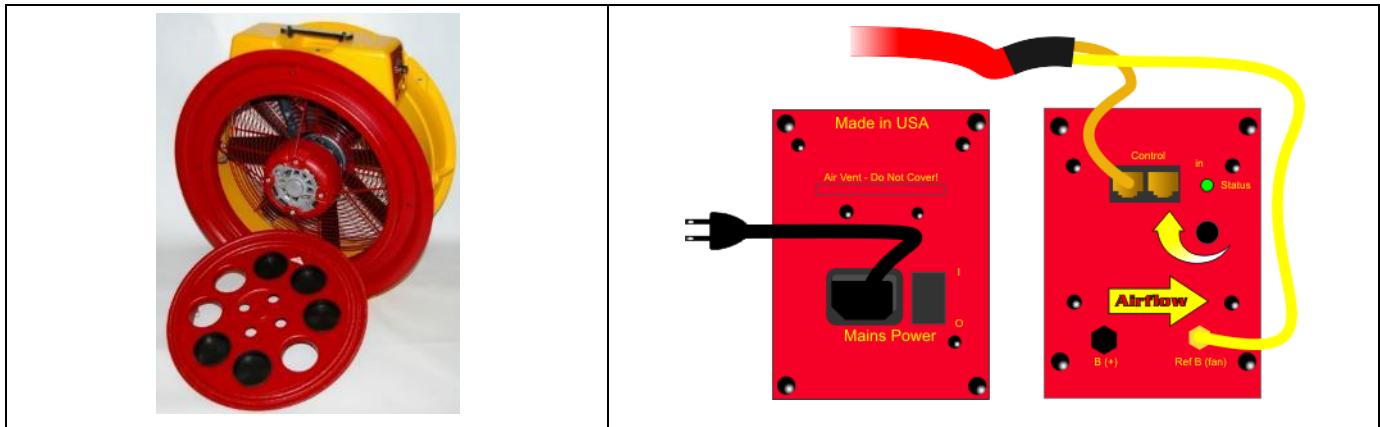
Figure 12: Model 1000 fan with two electrical plates containing power connection and switch, dual Control Ports and manual speed knob.
