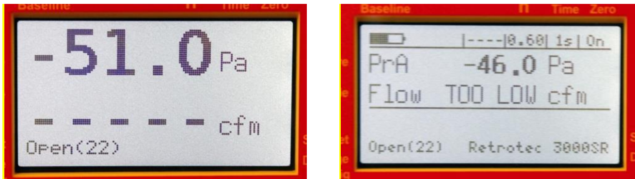
Figure 31: DM-2 can't display flow reading because of back pressure.
