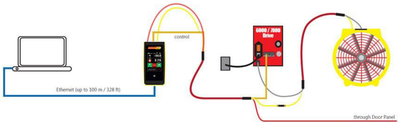
Figure 5. Connections between a 6000 / 7000 Door Fan, Drive, DM32 gauge, and laptop. Dimensions are not shown to scale.
