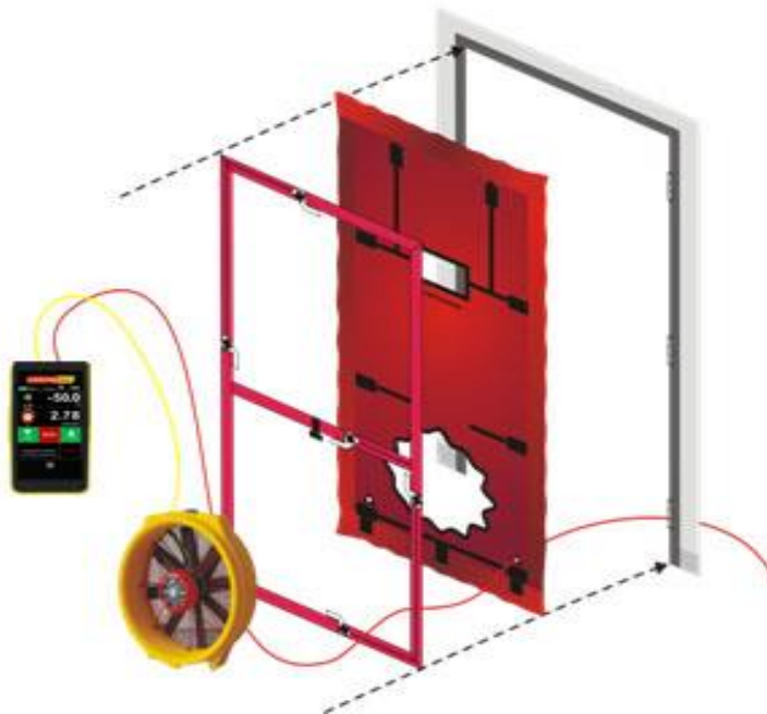
Figure 1: The breakdown of a typical Door Fan system.
